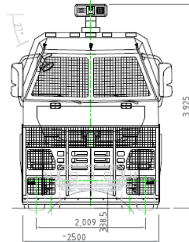
Water Riot Control Vehicle
